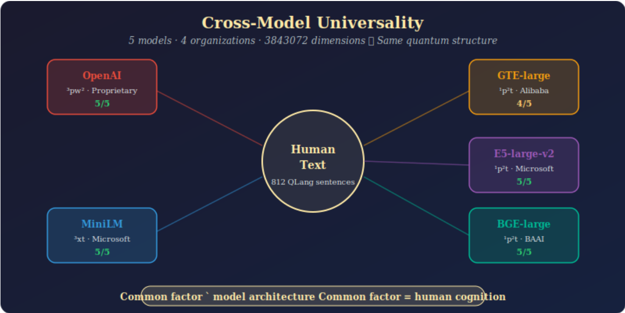
Figure 7: 10-universality
