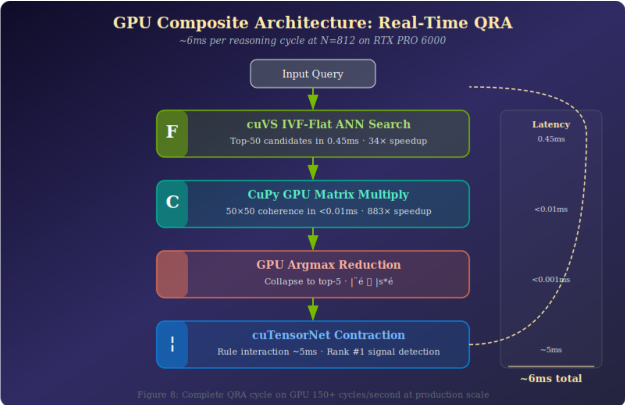
Figure 8: 08-gpu-composite
