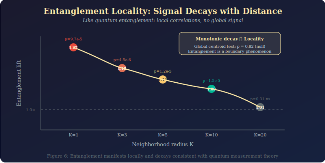
Figure 5: 06-entanglement-locality
