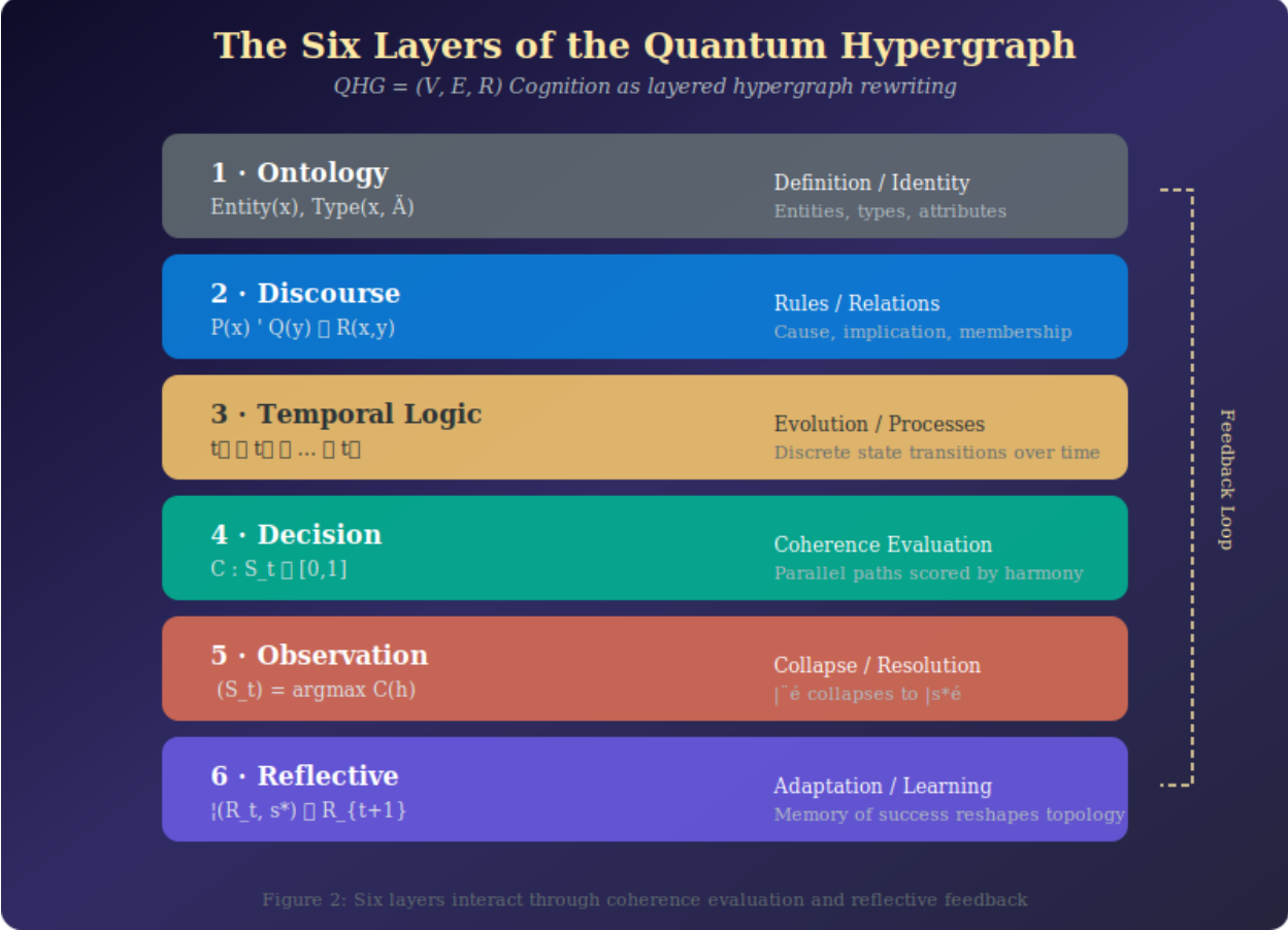
Figure 1: 02-six-layers
