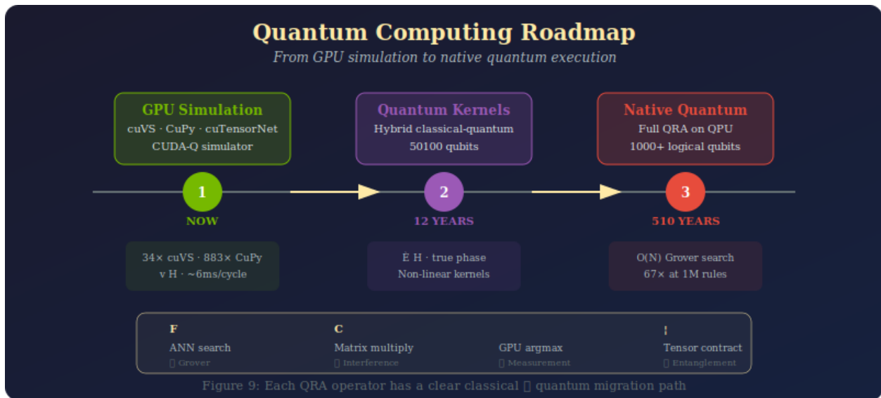
Figure 9: 09-quantum-roadmap
