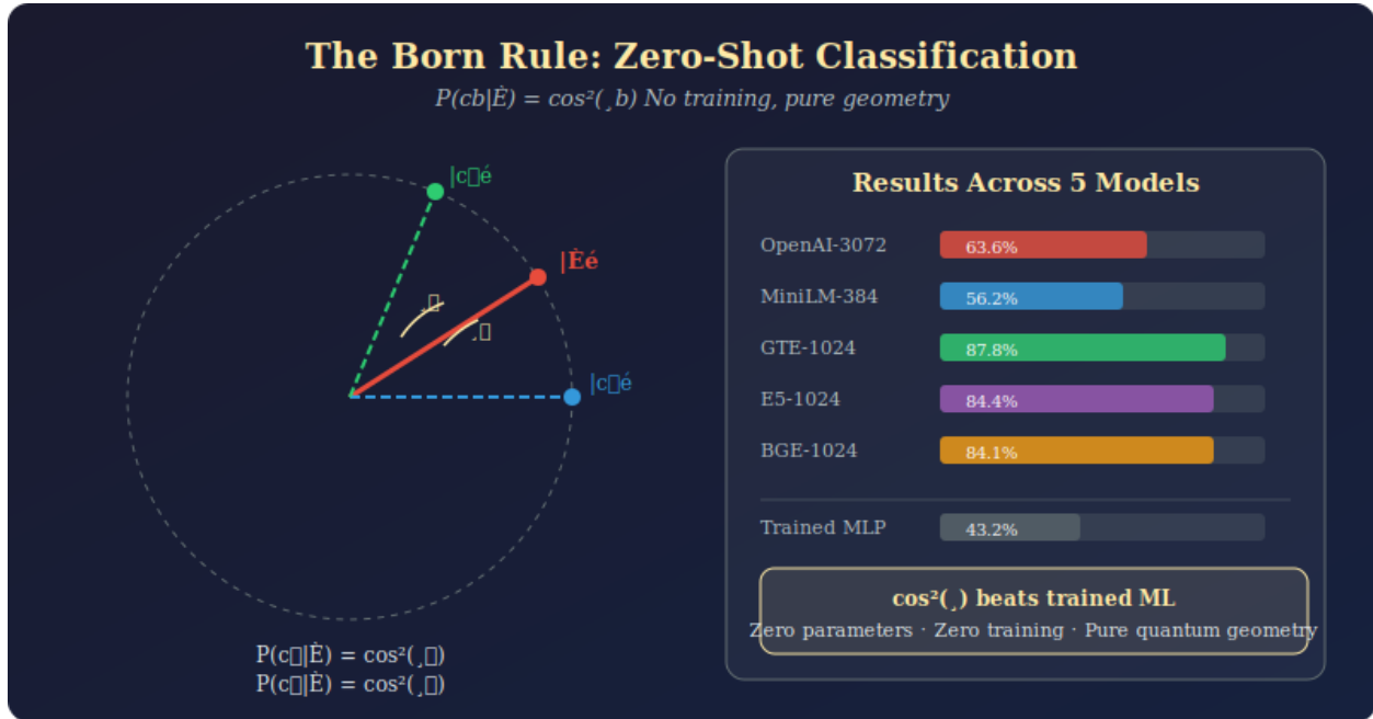
Figure 6: 04-born-rule
