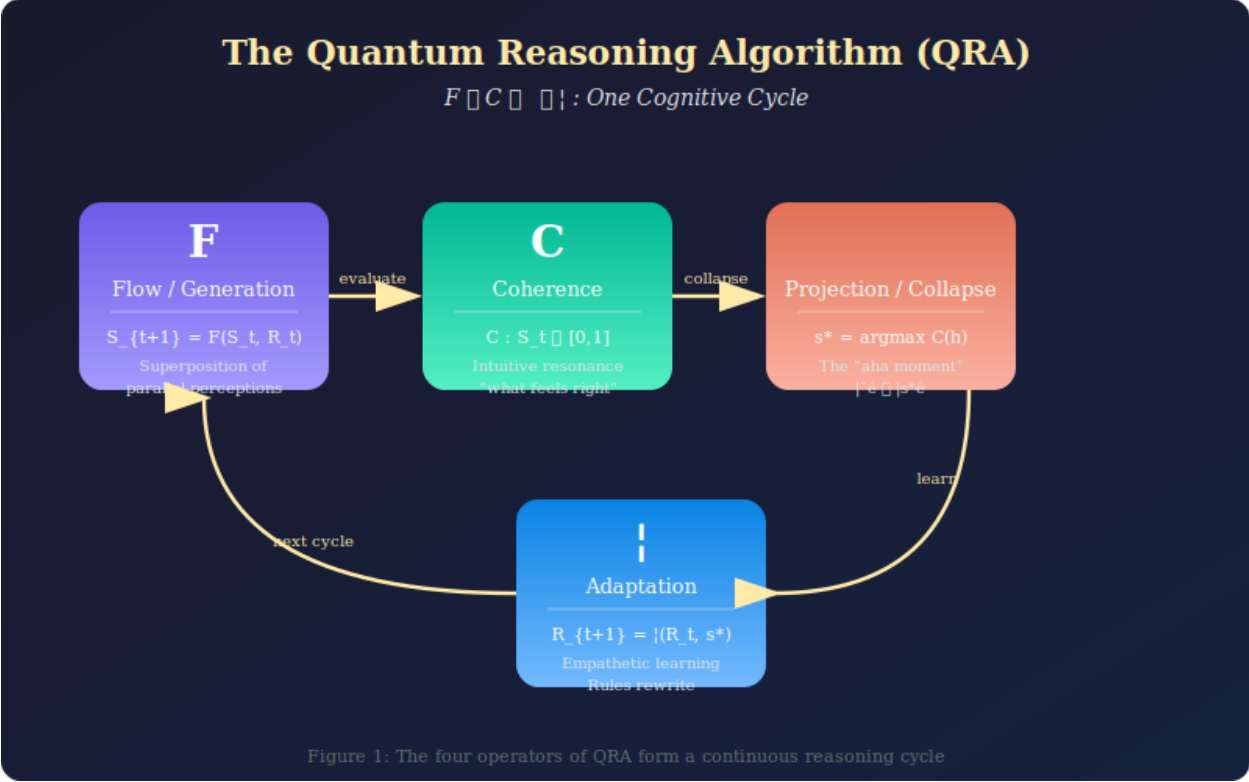
Figure 2: 01-qra-cycle
