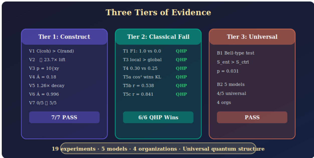
Figure 3: 07-three-tiers
